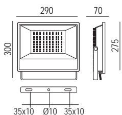
LED Virgola 50W
