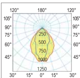
40°/80° Ovale diffondente - Oval flood
