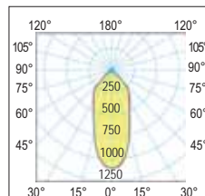
40° Intermedio - Medium
