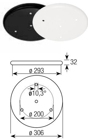
ROSONE TONDO Ø 305 - 4 FORI ROUND CEILING ROSE Ø 305 - 4 HOLES
