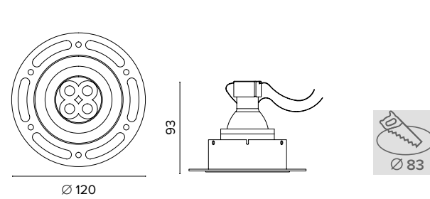
0698 TOSHIBA GU10 tondo / round
